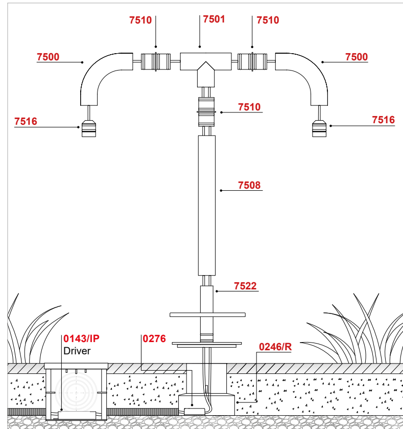
I drivers, da ordinare separatamente, devono essere collocati in remoto The drivers, to be ordered separately, must be placed remotely
